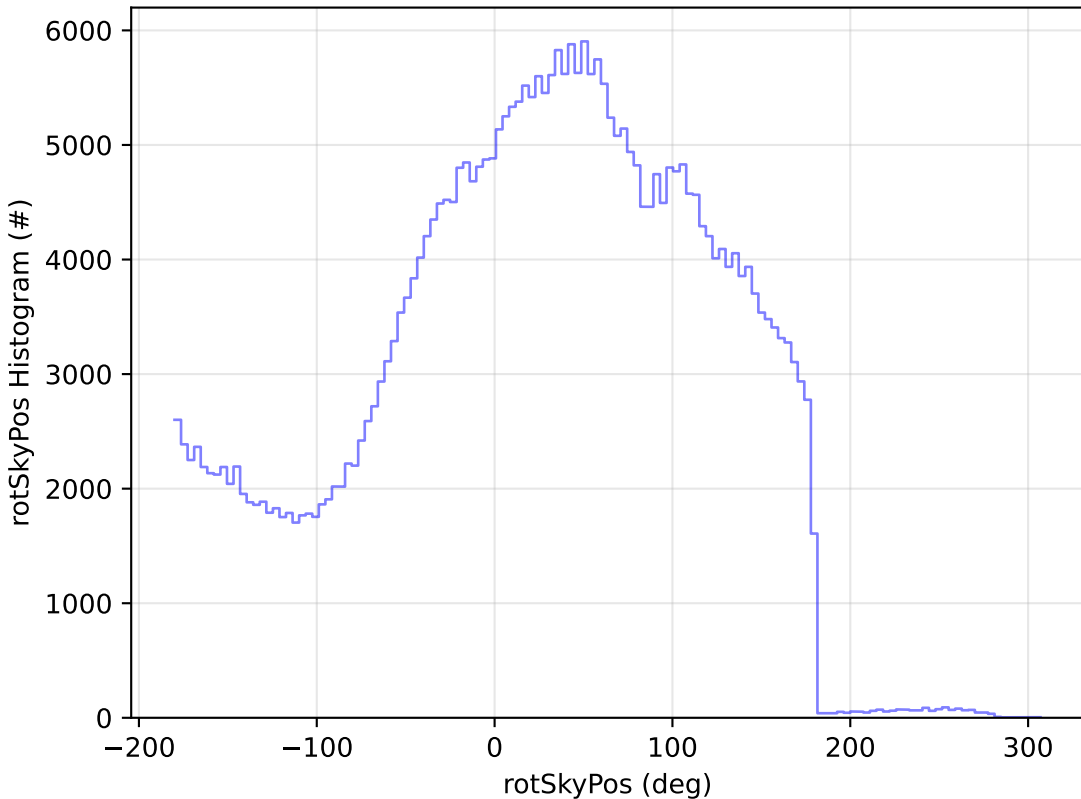
baseline_v3.5_10yrs WFD y band: rotSkyPos Histogram
