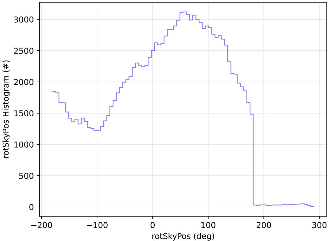
baseline_v3.5_10yrs WFD u band: rotSkyPos Histogram
