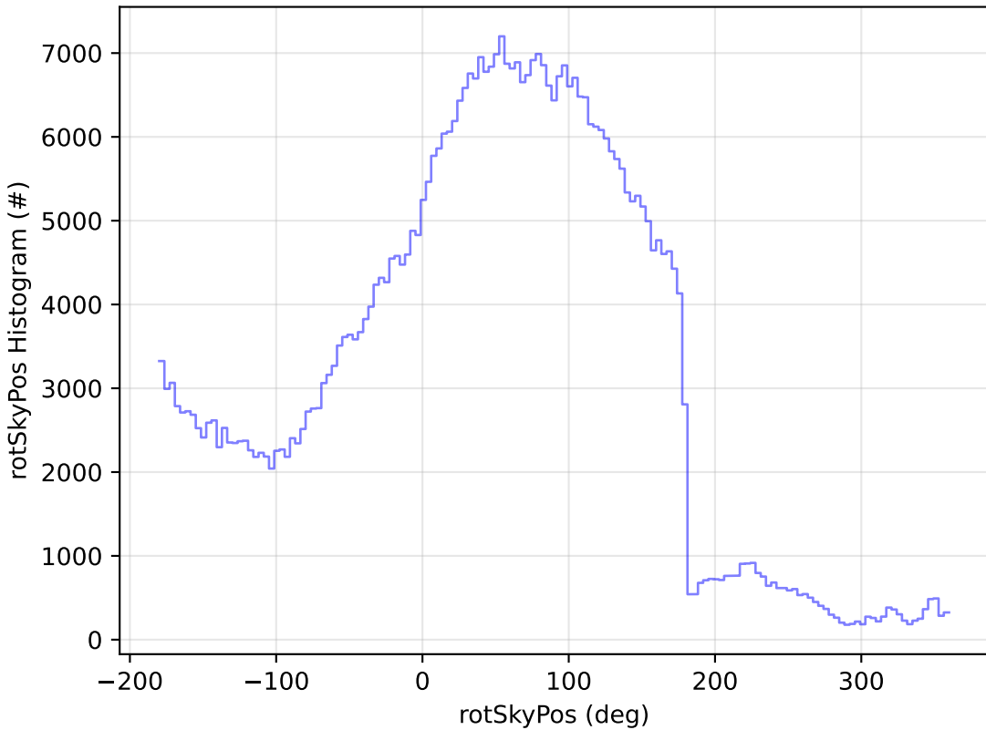
baseline_v3.5_10yrs WFD r band: rotSkyPos Histogram
