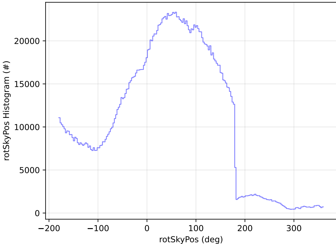
baseline_v3.5_10yrs WFD all bands: rotSkyPos Histogram
