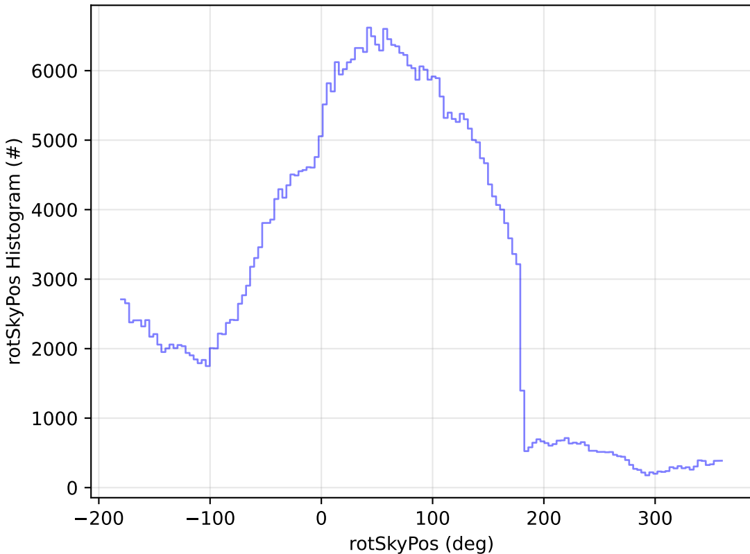
baseline_v3.5_10yrs All sky z band: rotSkyPos Histogram
