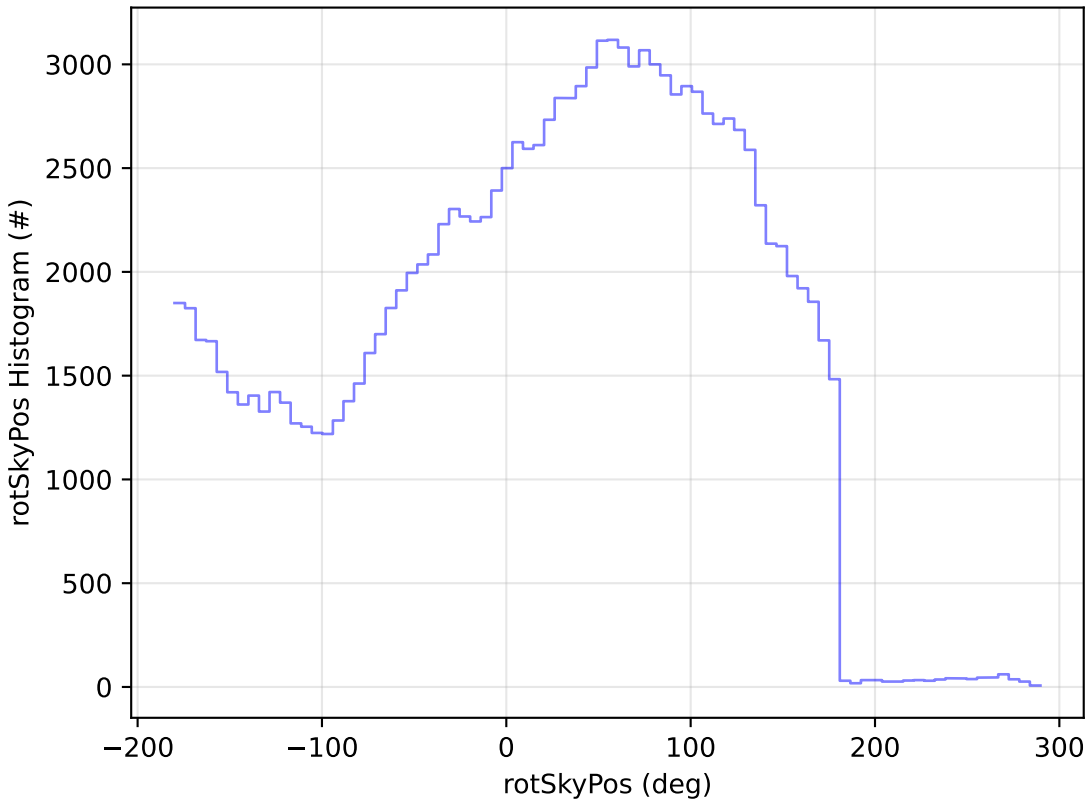
baseline_v3.5_10yrs All sky u band: rotSkyPos Histogram
