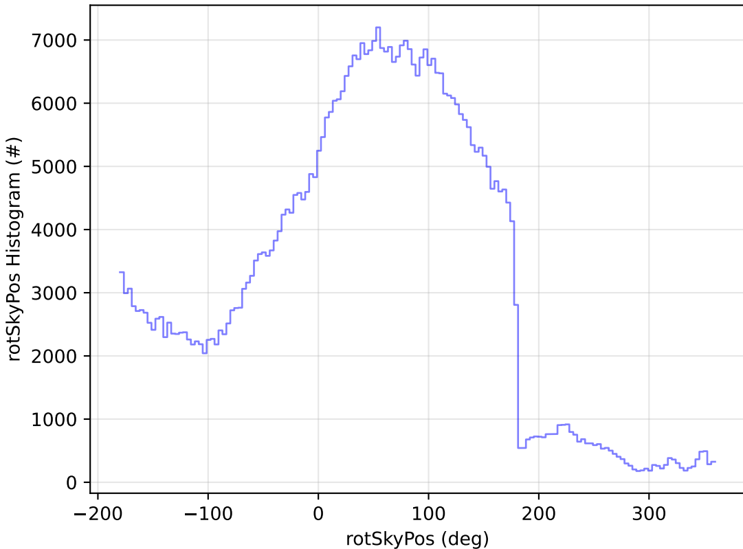
baseline_v3.5_10yrs All sky r band: rotSkyPos Histogram
