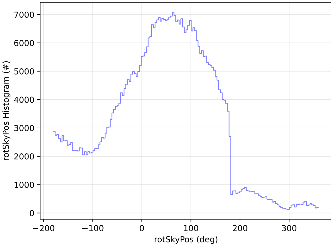
baseline_v3.5_10yrs All sky i band: rotSkyPos Histogram
