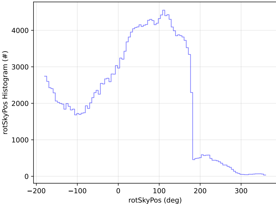
baseline_v3.5_10yrs All sky g band: rotSkyPos Histogram
