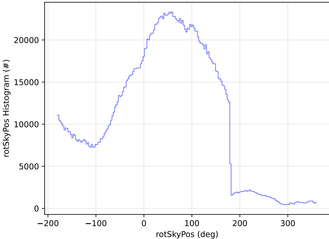
baseline_v3.5_10yrs All sky all bands: rotSkyPos Histogram
