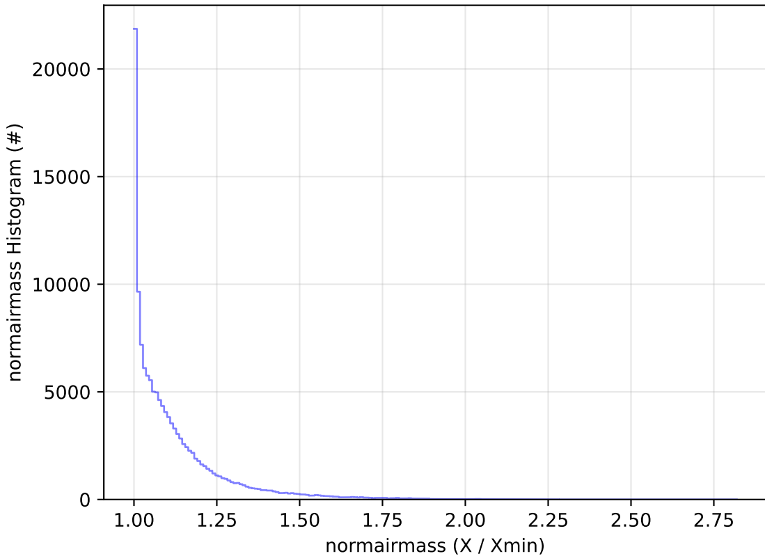
baseline_v3.5_10yrs WFD u band: normairmass Histogram
