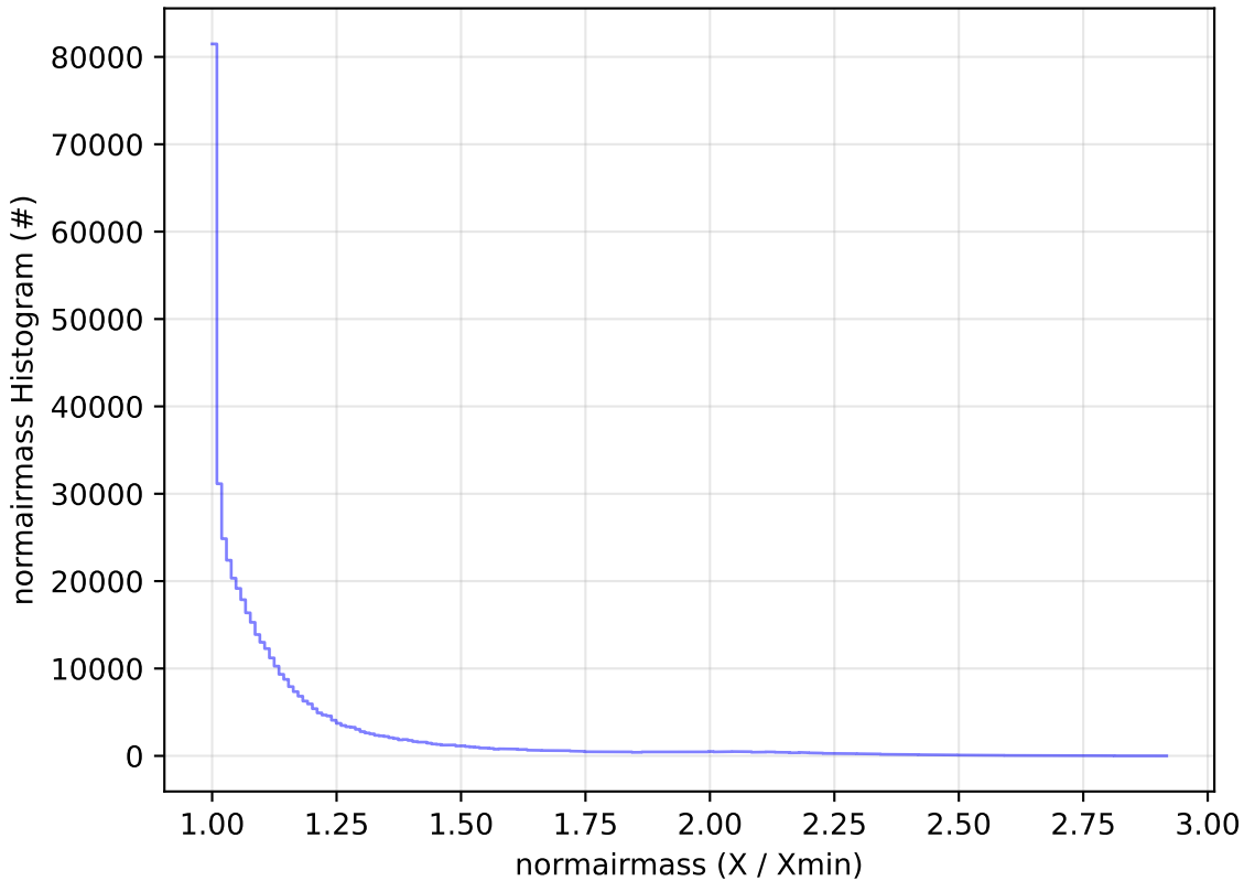
baseline_v3.5_10yrs WFD i band: normairmass Histogram
