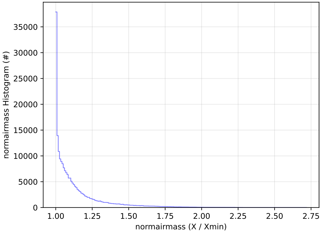
baseline_v3.5_10yrs WFD g band: normairmass Histogram
