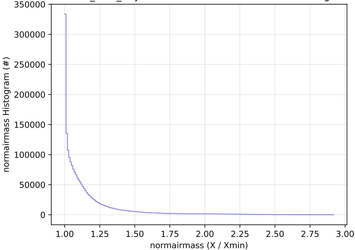
baseline_v3.5_10yrs WFD all bands: normairmass Histogram
