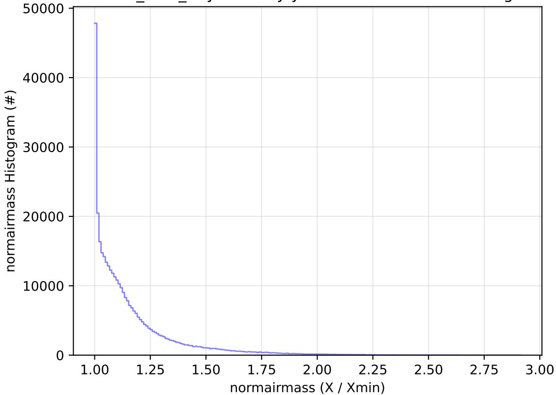
baseline_v3.5_10yrs All sky y band: normairmass Histogram
