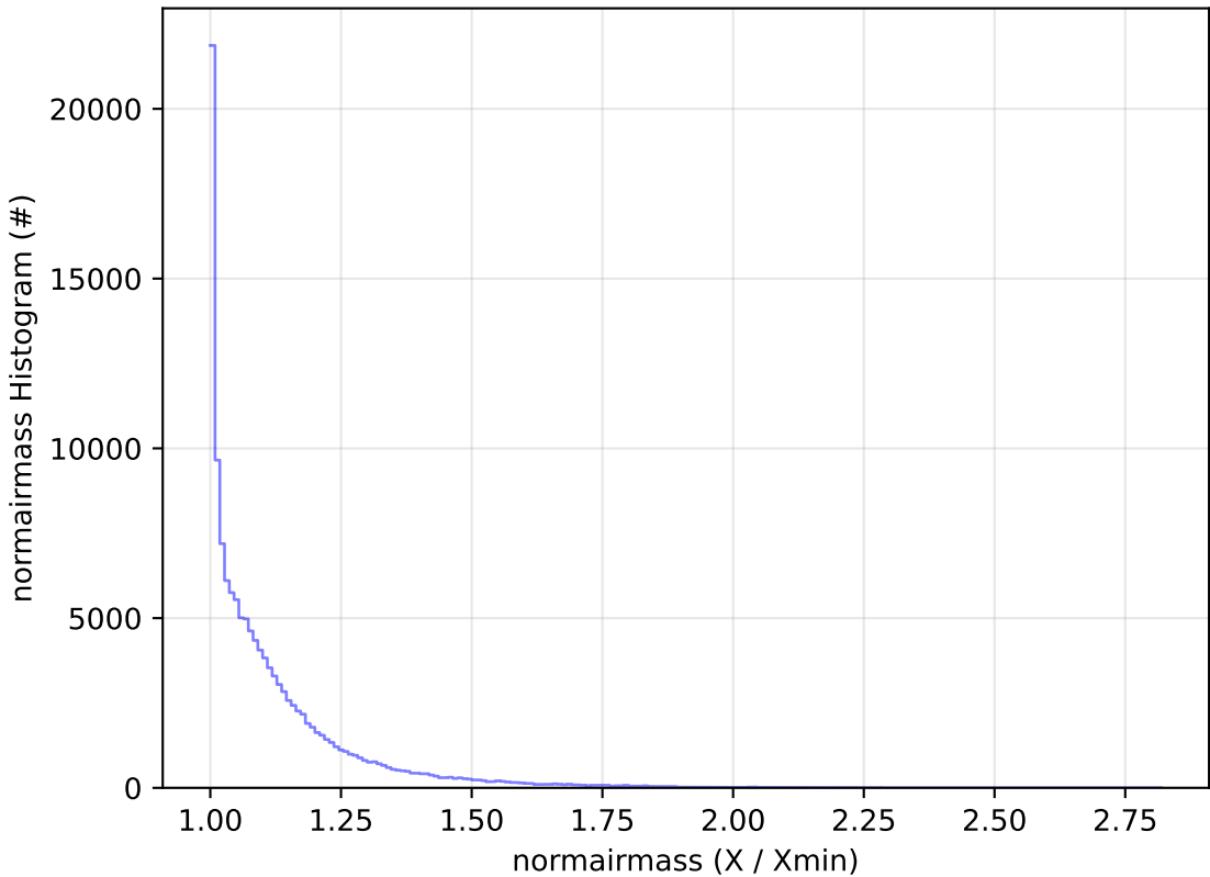
baseline_v3.5_10yrs All sky u band: normairmass Histogram
