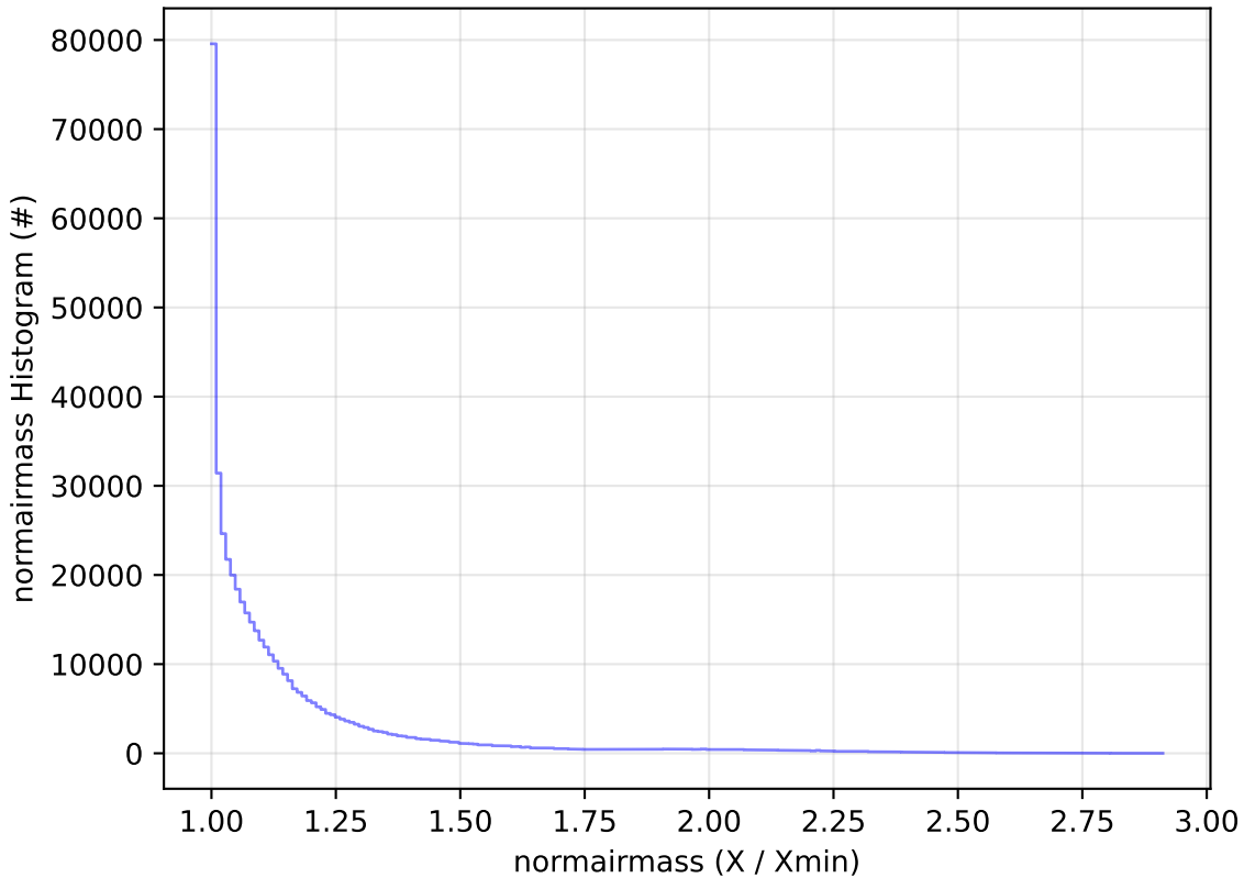
baseline_v3.5_10yrs All sky r band: normairmass Histogram
