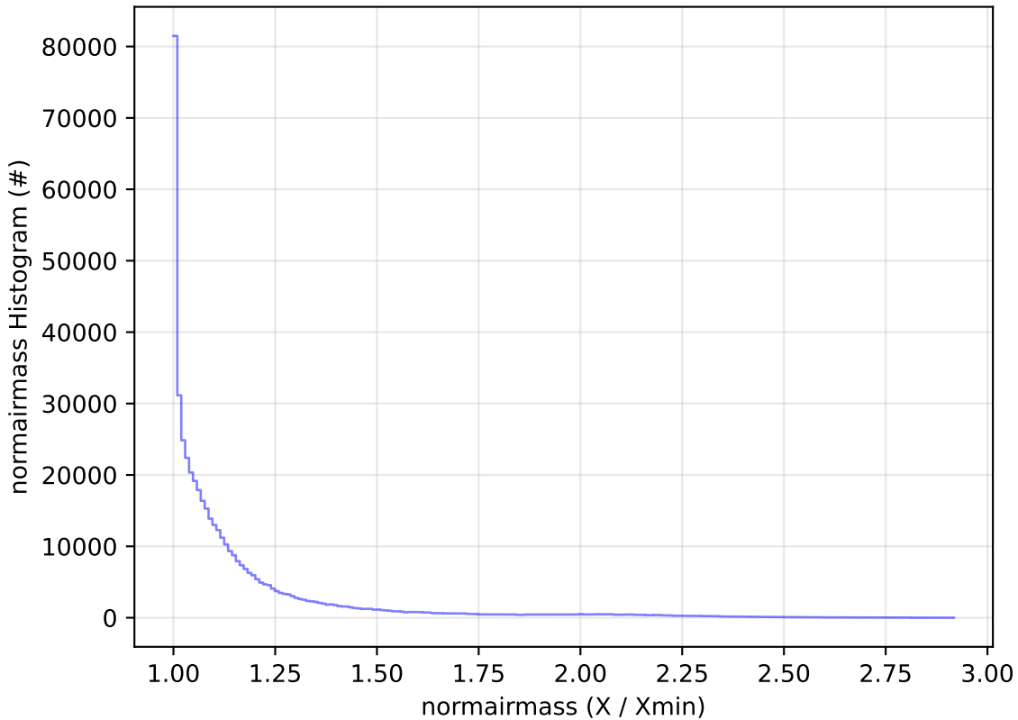
baseline_v3.5_10yrs All sky i band: normairmass Histogram
