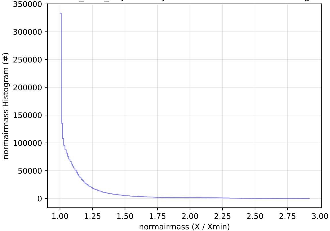
baseline_v3.5_10yrs All sky all bands: normairmass Histogram
