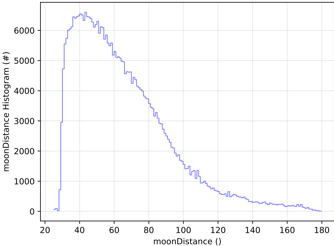
baseline_v3.5_10yrs WFD y band: moonDistance Histogram
