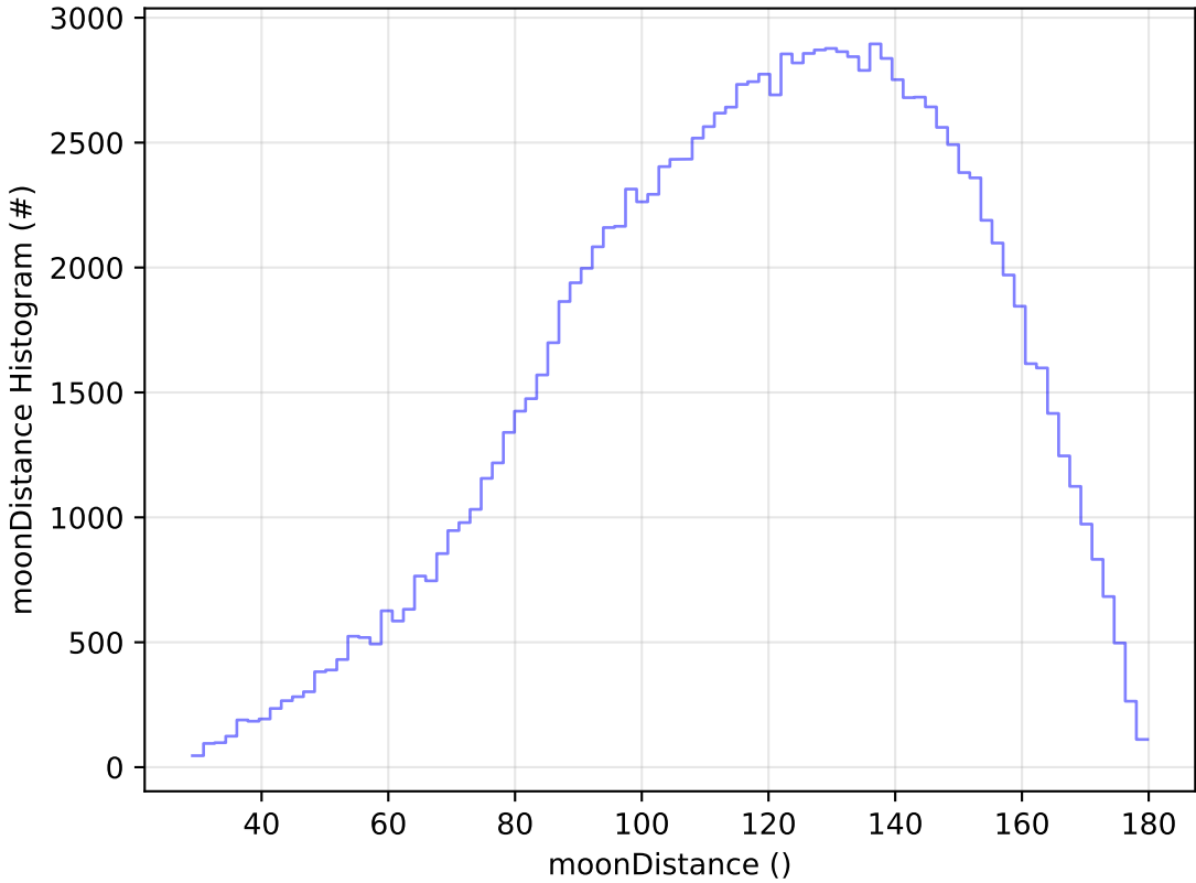
baseline_v3.5_10yrs WFD u band: moonDistance Histogram
