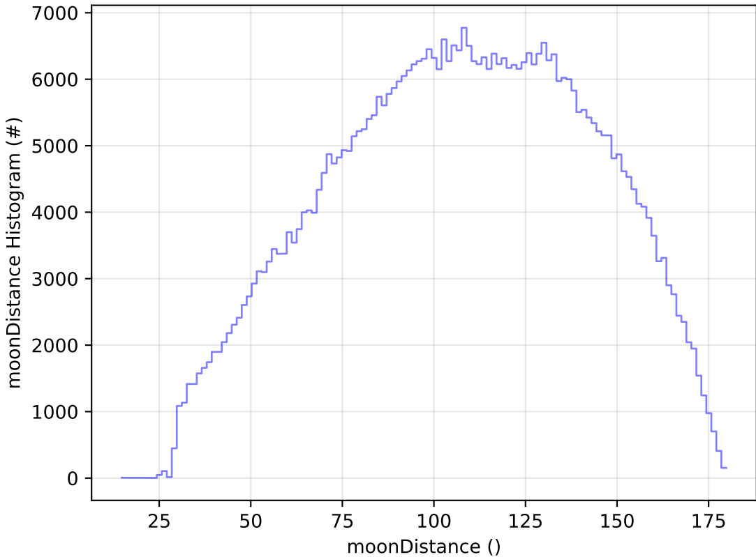
baseline_v3.5_10yrs WFD r band: moonDistance Histogram
