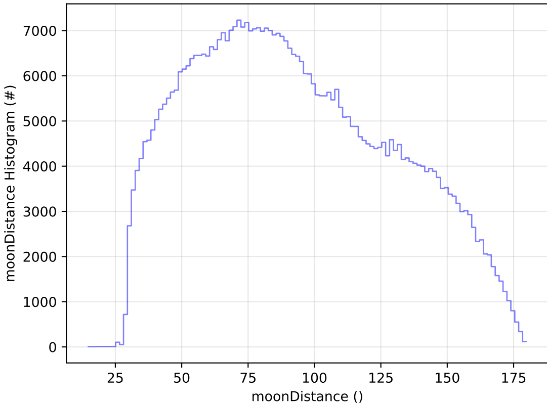
baseline_v3.5_10yrs WFD i band: moonDistance Histogram
