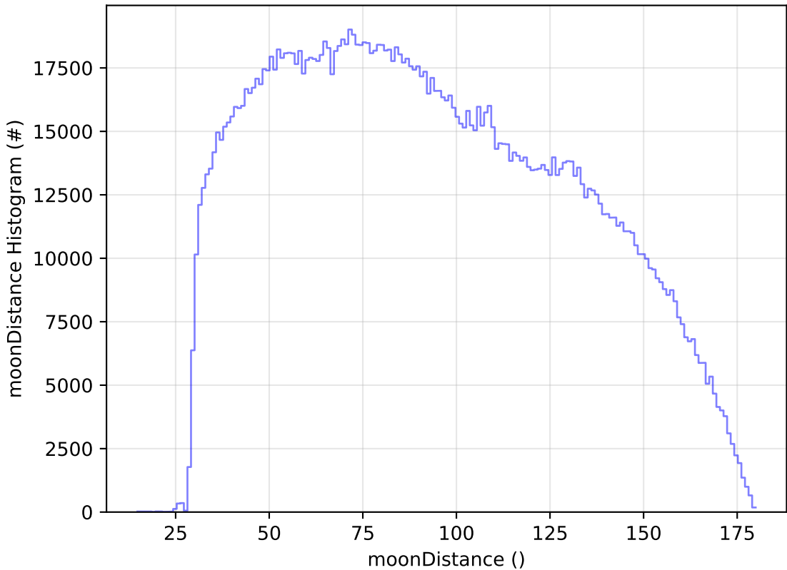
baseline_v3.5_10yrs WFD all bands: moonDistance Histogram
