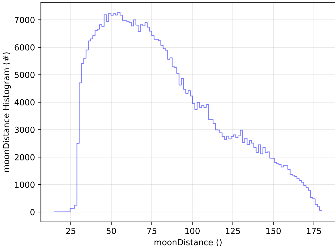
baseline_v3.5_10yrs All sky z band: moonDistance Histogram
