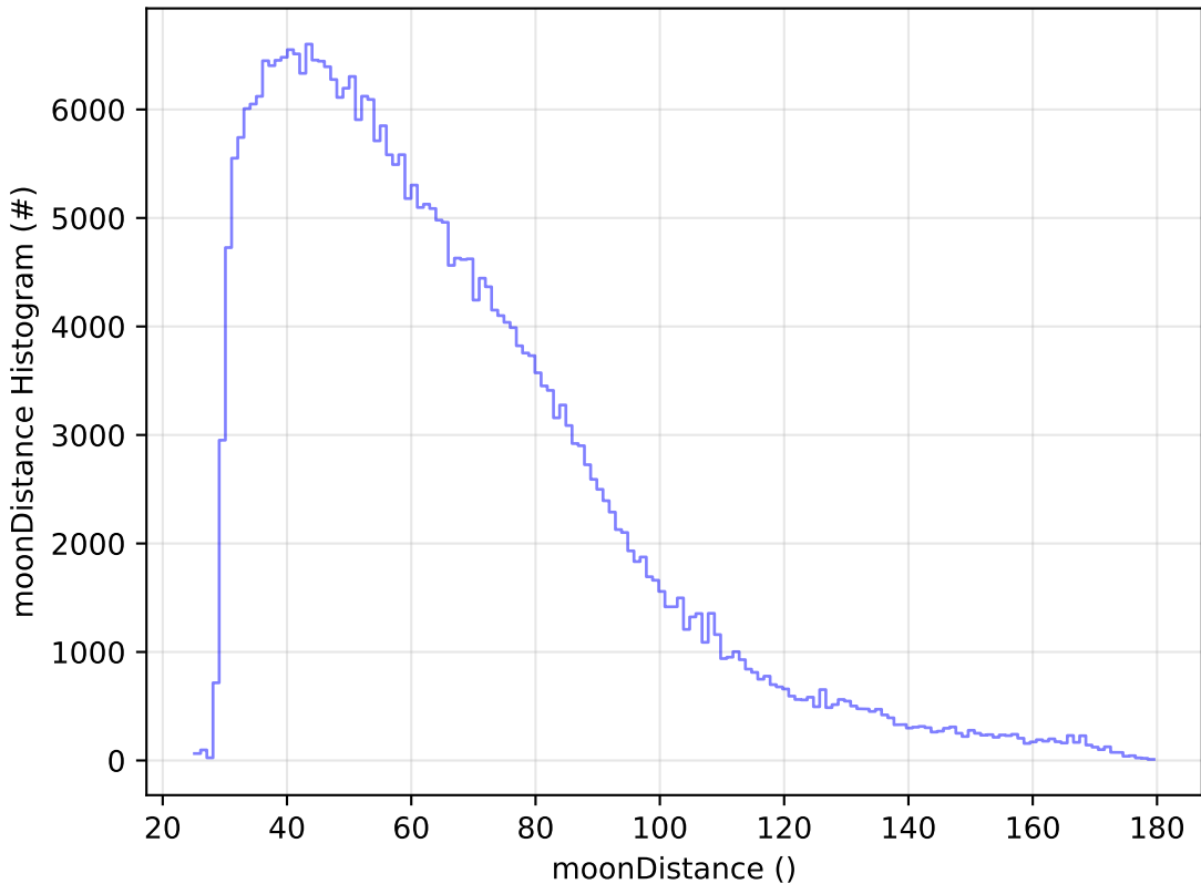
baseline_v3.5_10yrs All sky y band: moonDistance Histogram
