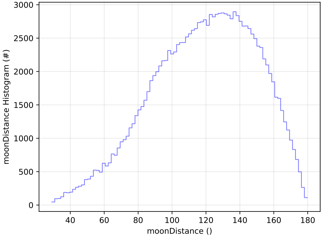
baseline_v3.5_10yrs All sky u band: moonDistance Histogram
