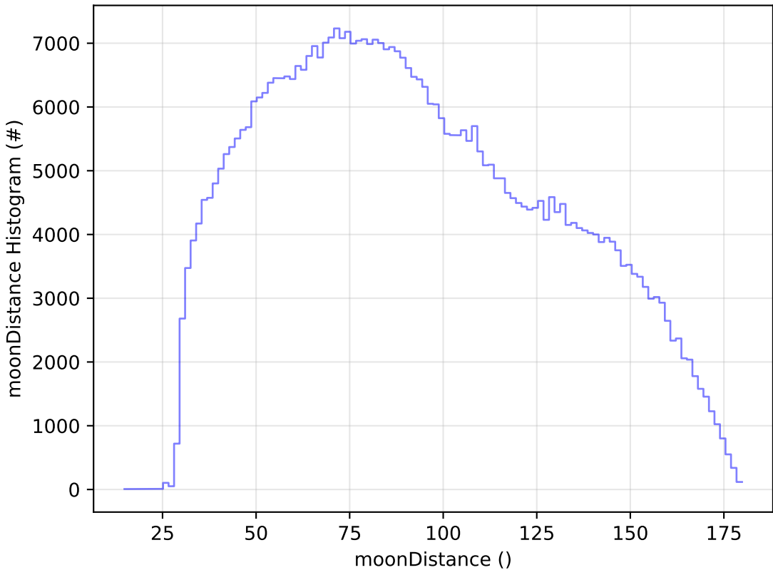
baseline_v3.5_10yrs All sky i band: moonDistance Histogram
