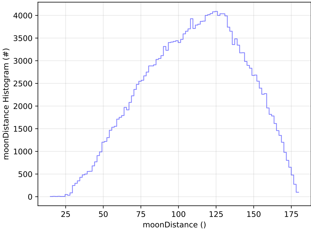
baseline_v3.5_10yrs All sky g band: moonDistance Histogram
