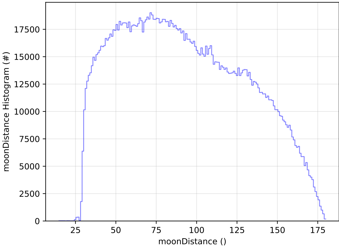
baseline_v3.5_10yrs All sky all bands: moonDistance Histogram
