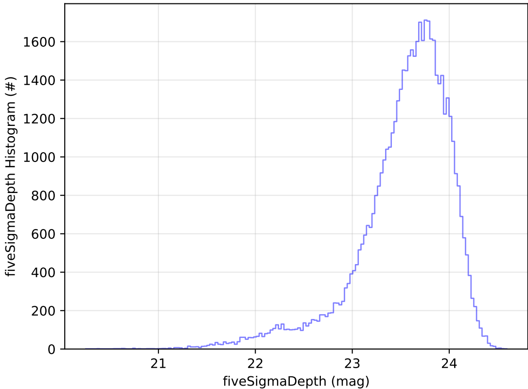
baseline_v3.5_10yrs Yr 1 i band: fiveSigmaDepth Histogram
