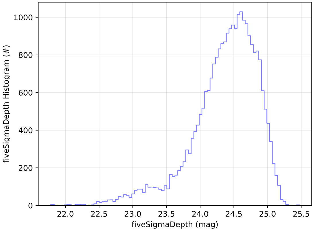
baseline_v3.5_10yrs Yr 1 g band: fiveSigmaDepth Histogram
