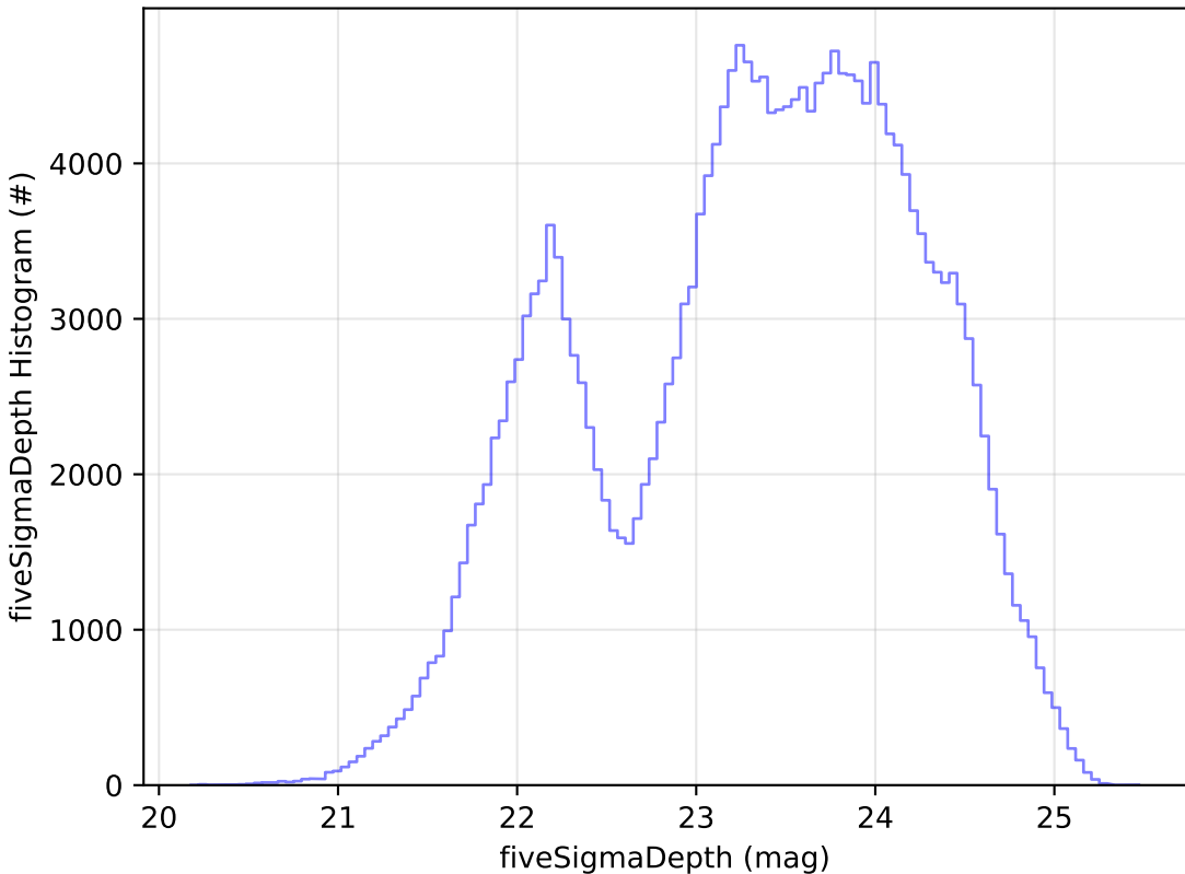
baseline_v3.5_10yrs Yr 1 all bands: fiveSigmaDepth Histogram
