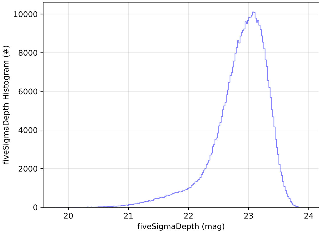
baseline_v3.5_10yrs WFD z band: fiveSigmaDepth Histogram
