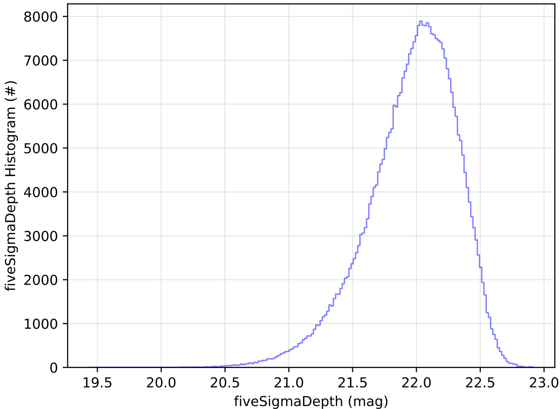
baseline_v3.5_10yrs WFD y band: fiveSigmaDepth Histogram
