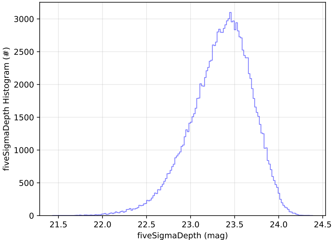
baseline_v3.5_10yrs WFD u band: fiveSigmaDepth Histogram
