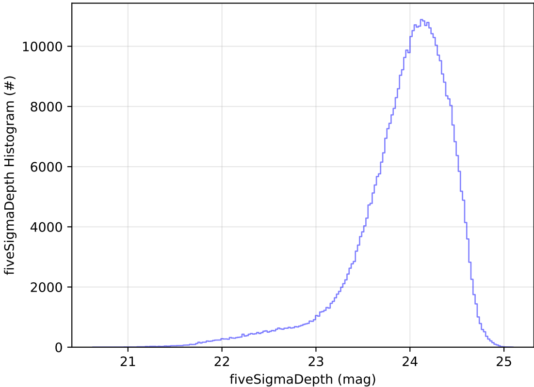
baseline_v3.5_10yrs WFD r band: fiveSigmaDepth Histogram
