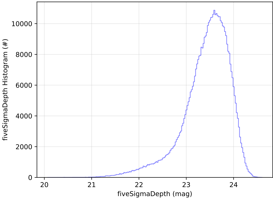
baseline_v3.5_10yrs WFD i band: fiveSigmaDepth Histogram
