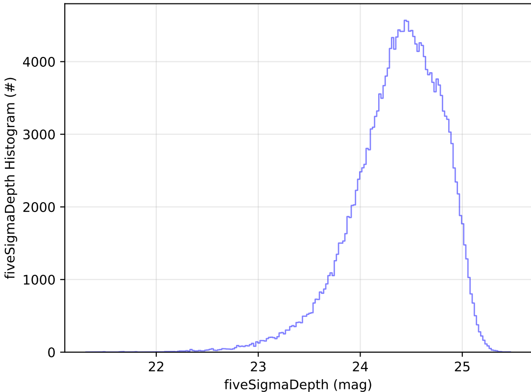
baseline_v3.5_10yrs WFD g band: fiveSigmaDepth Histogram
