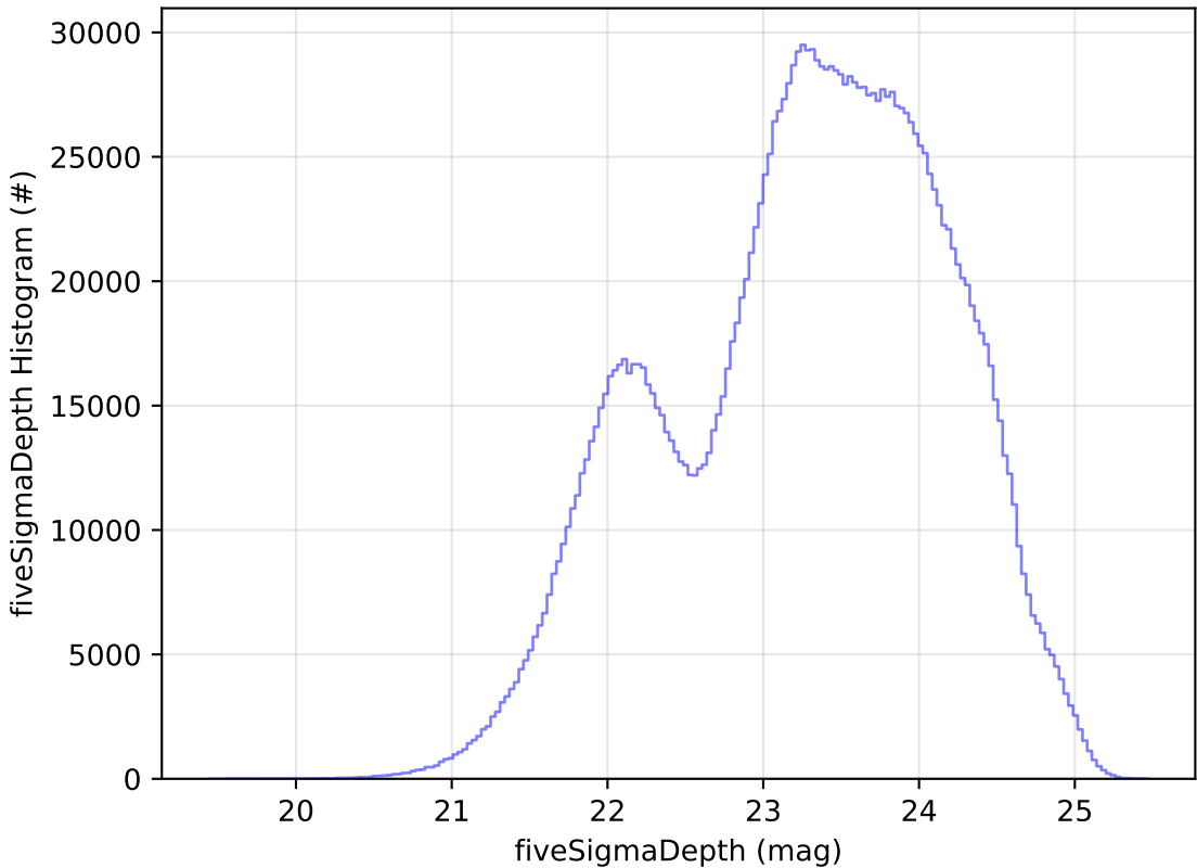
baseline_v3.5_10yrs WFD all bands: fiveSigmaDepth Histogram
