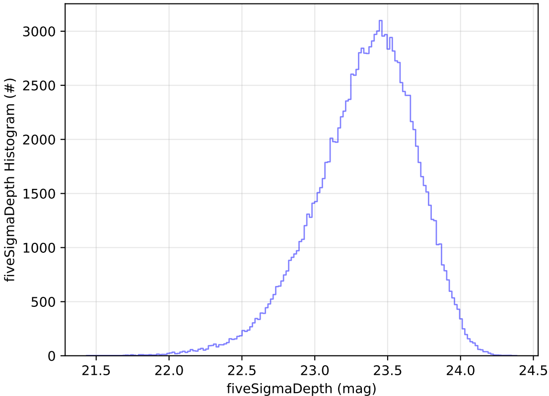
baseline_v3.5_10yrs All sky u band: fiveSigmaDepth Histogram
