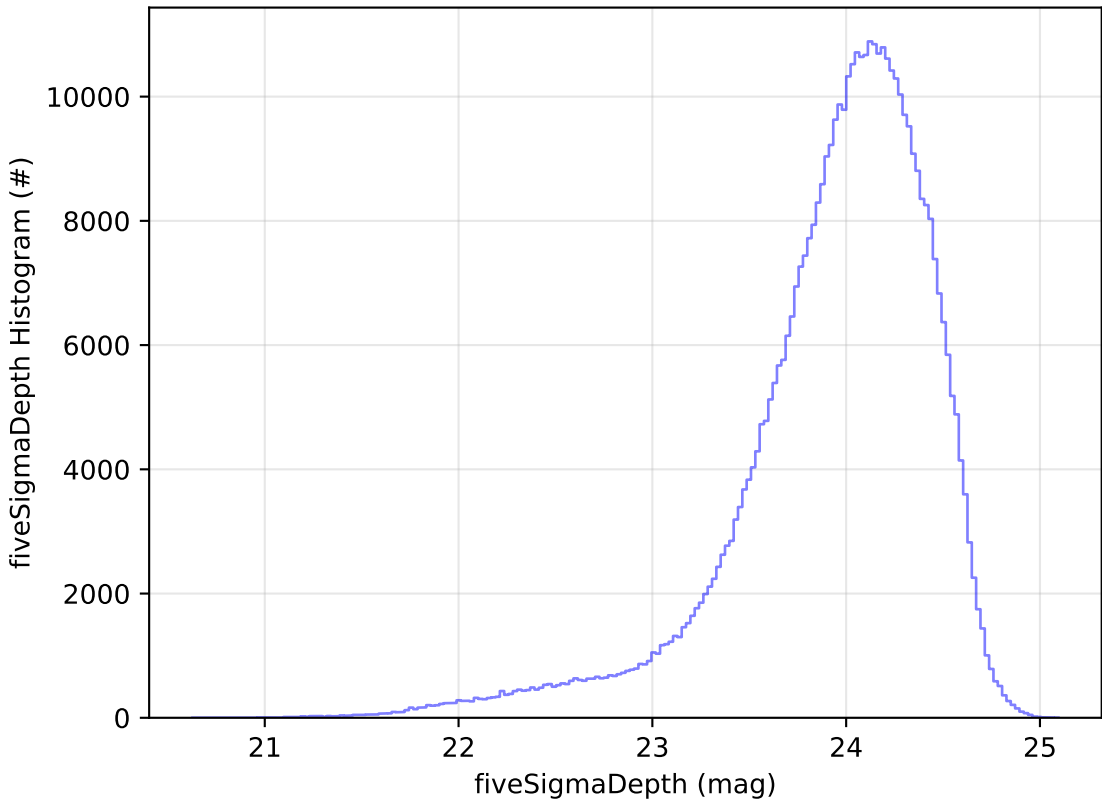
baseline_v3.5_10yrs All sky r band: fiveSigmaDepth Histogram
