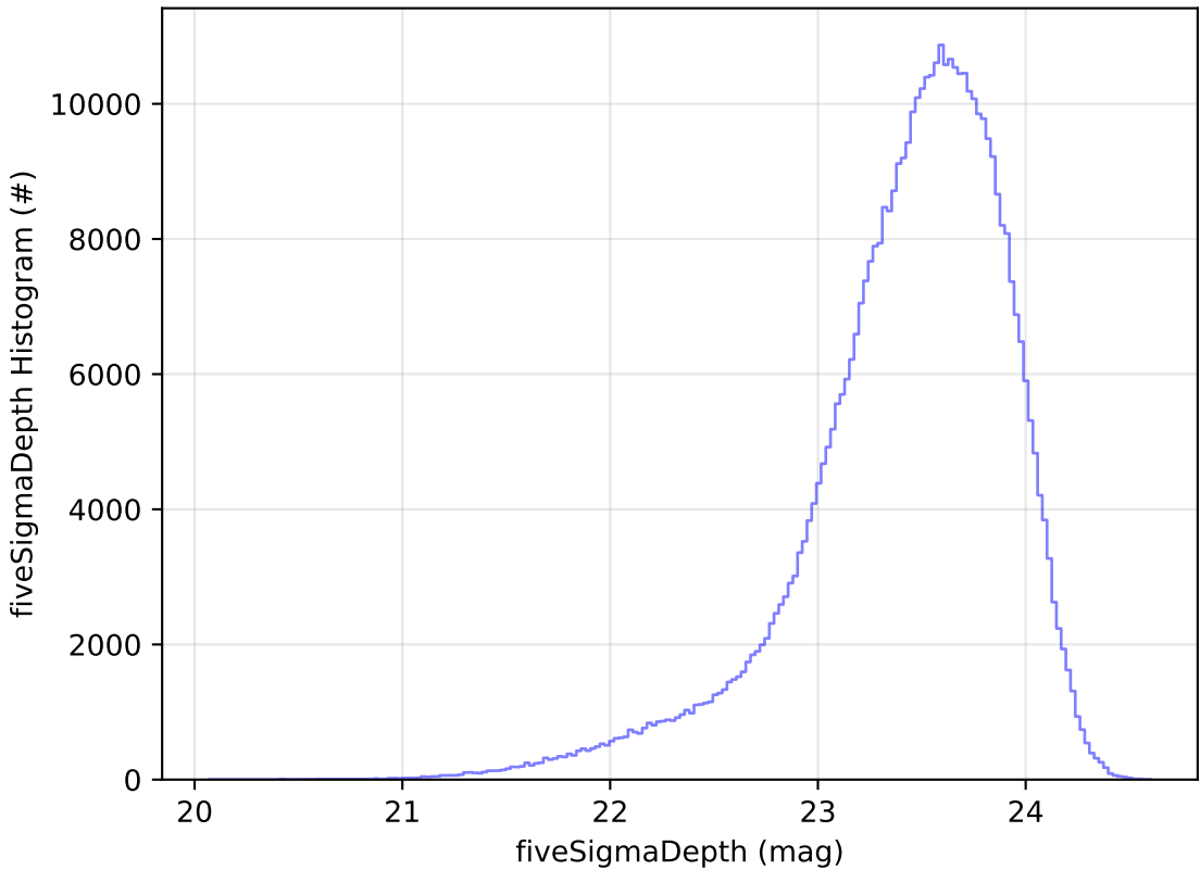
baseline_v3.5_10yrs All sky i band: fiveSigmaDepth Histogram
