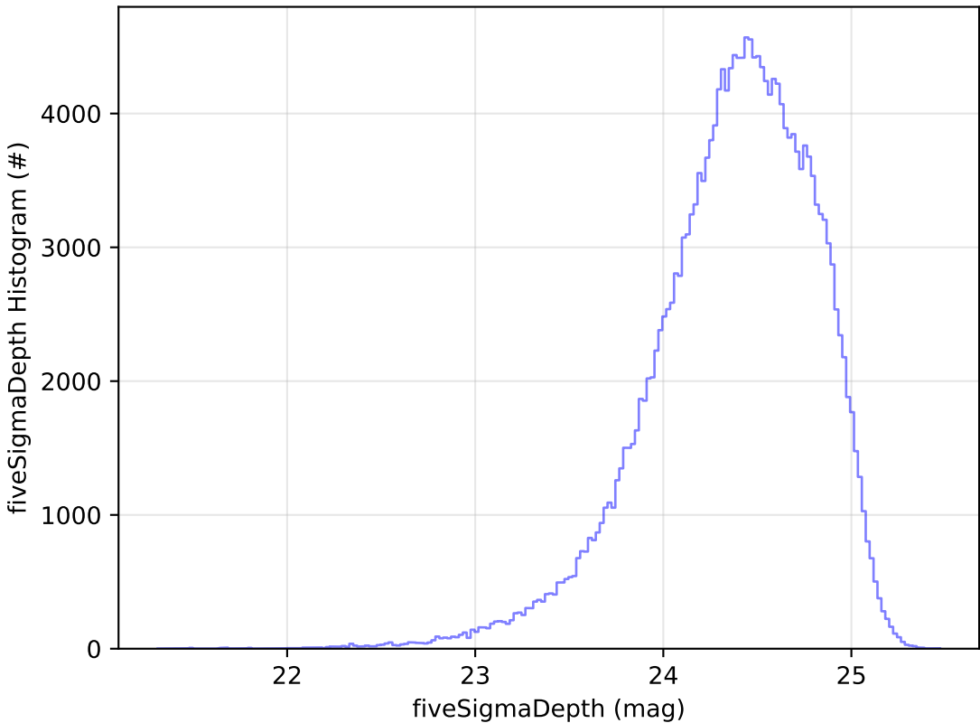
baseline_v3.5_10yrs All sky g band: fiveSigmaDepth Histogram
