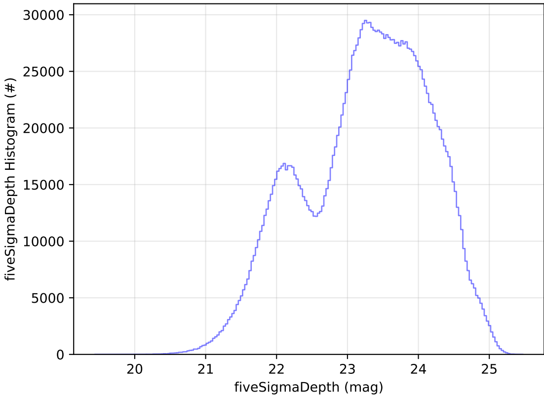
baseline_v3.5_10yrs All sky all bands: fiveSigmaDepth Histogram
