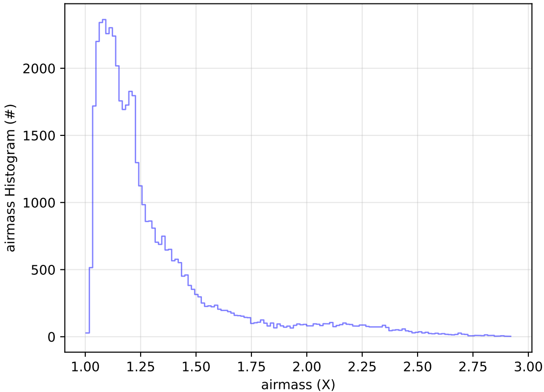
baseline_v3.5_10yrs Yr 1 z band: airmass Histogram
