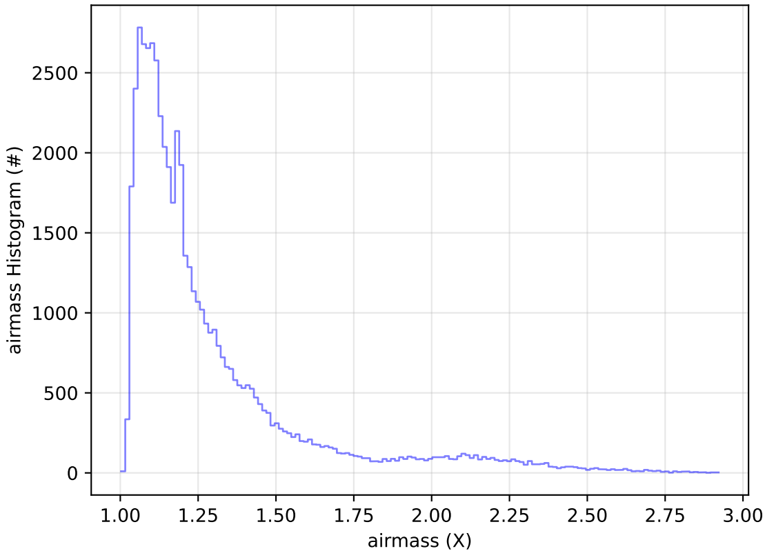
baseline_v3.5_10yrs Yr 1 i band: airmass Histogram
