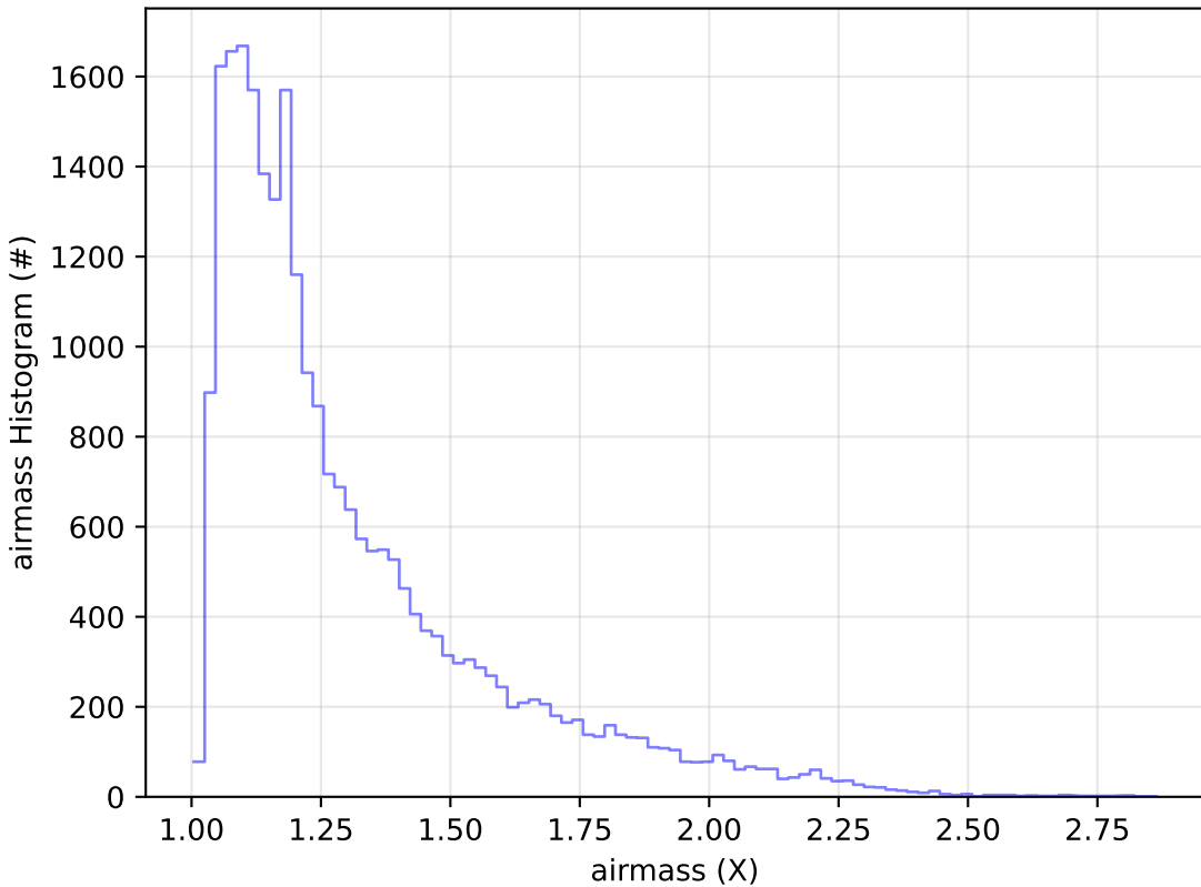
baseline_v3.5_10yrs Yr 1 g band: airmass Histogram
