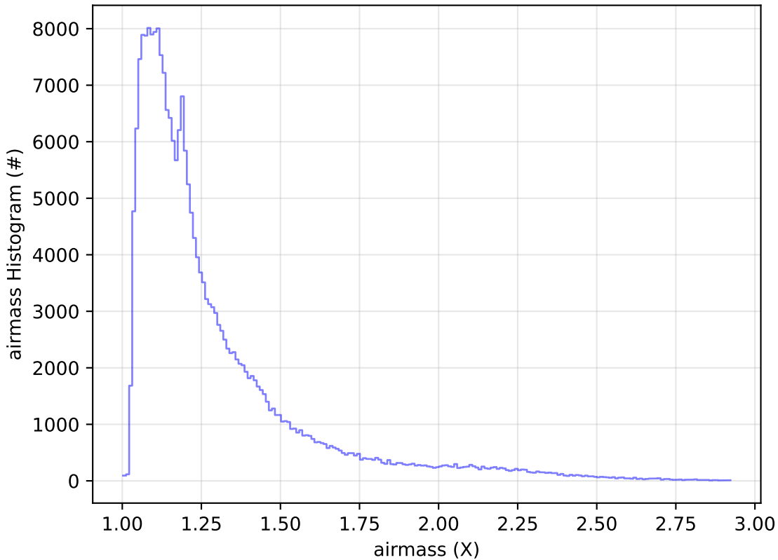
baseline_v3.5_10yrs Yr 1 all bands: airmass Histogram
