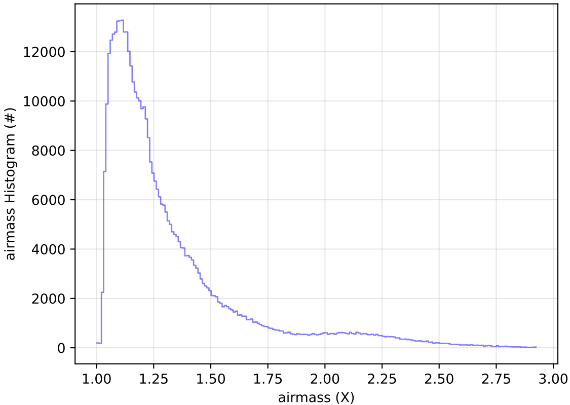
baseline_v3.5_10yrs WFD z band: airmass Histogram
